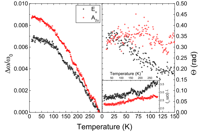
Figure 7. (Color online) Summary of the three fit parameters of the high energy phonon modes of the a -axis and c -axis to a Fano-shape resonance where \Delta\omega = \omega(T) - \omega(0) and \omega_0 is the oscillator's central frequency at room temperature.
