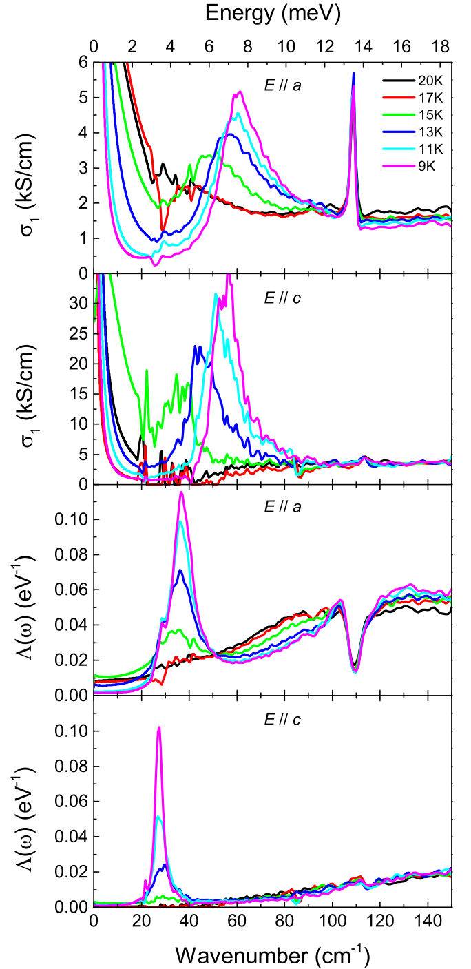
Figure 8. (Color online) Low energy optical conductivity (top panels) and loss function (bottom panels) at selected temperatures close and below T_{HO} for a -axis and c -axis polarizations.
