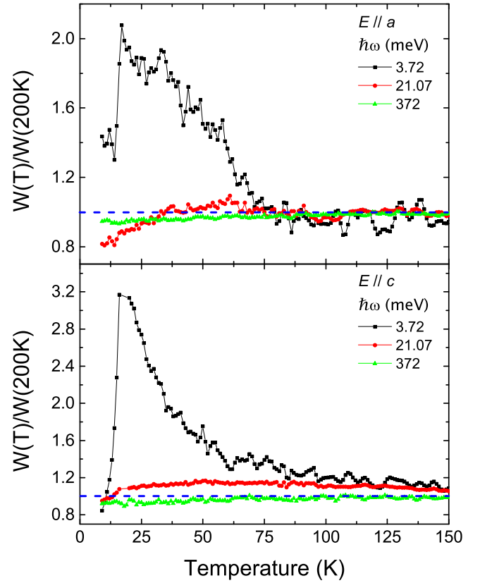
Figure 6. (Color online) normalized spectral weight obtained by integrating the conductivity from zero to the cut-off frequency \omega indicated in the figure legend for the a -axis (upper panel) and c -axis (lower panel) data. The spectral weights are normalized to W(200 \text{ K}) .
