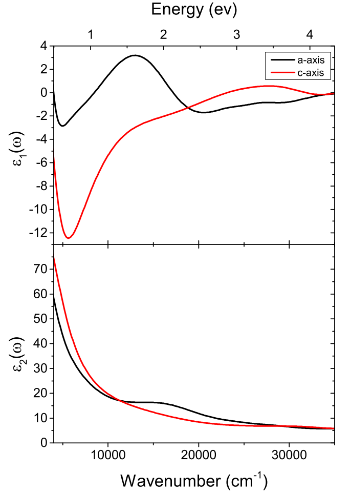
Figure 12. (Color online) The real (upper panel) and imaginary (lower panel) parts of the dielectric function \epsilon(\omega) a -axis (black) and c -axis (red) polarizations obtained from a fit to the Drude-Lorentz model and based on the ellipsometry measurements shown in Fig. 11.
