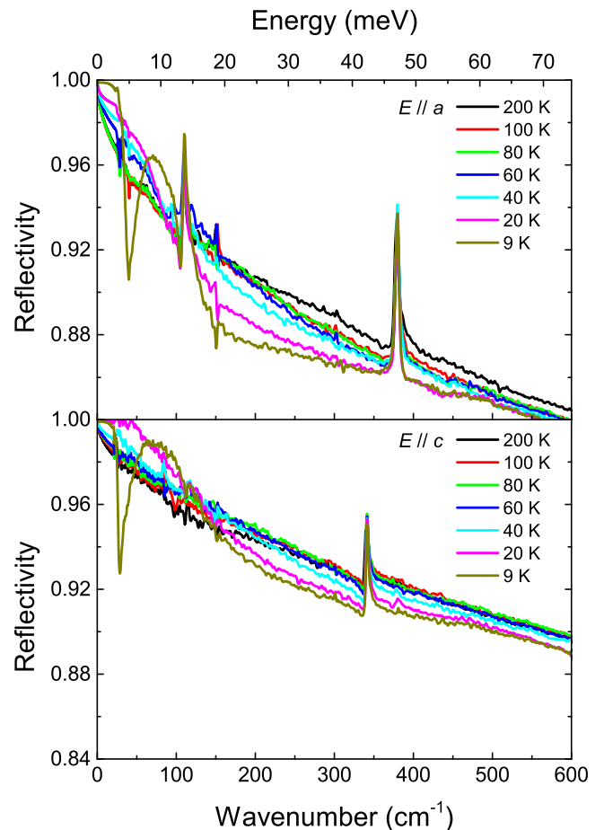
Figure 2. (Color online) Reflectivity of \text{URu}_2\text{Si}_2 single crystal in a -axis (upper panel) and c -axis (lower panel) polarizations for selected temperatures.
