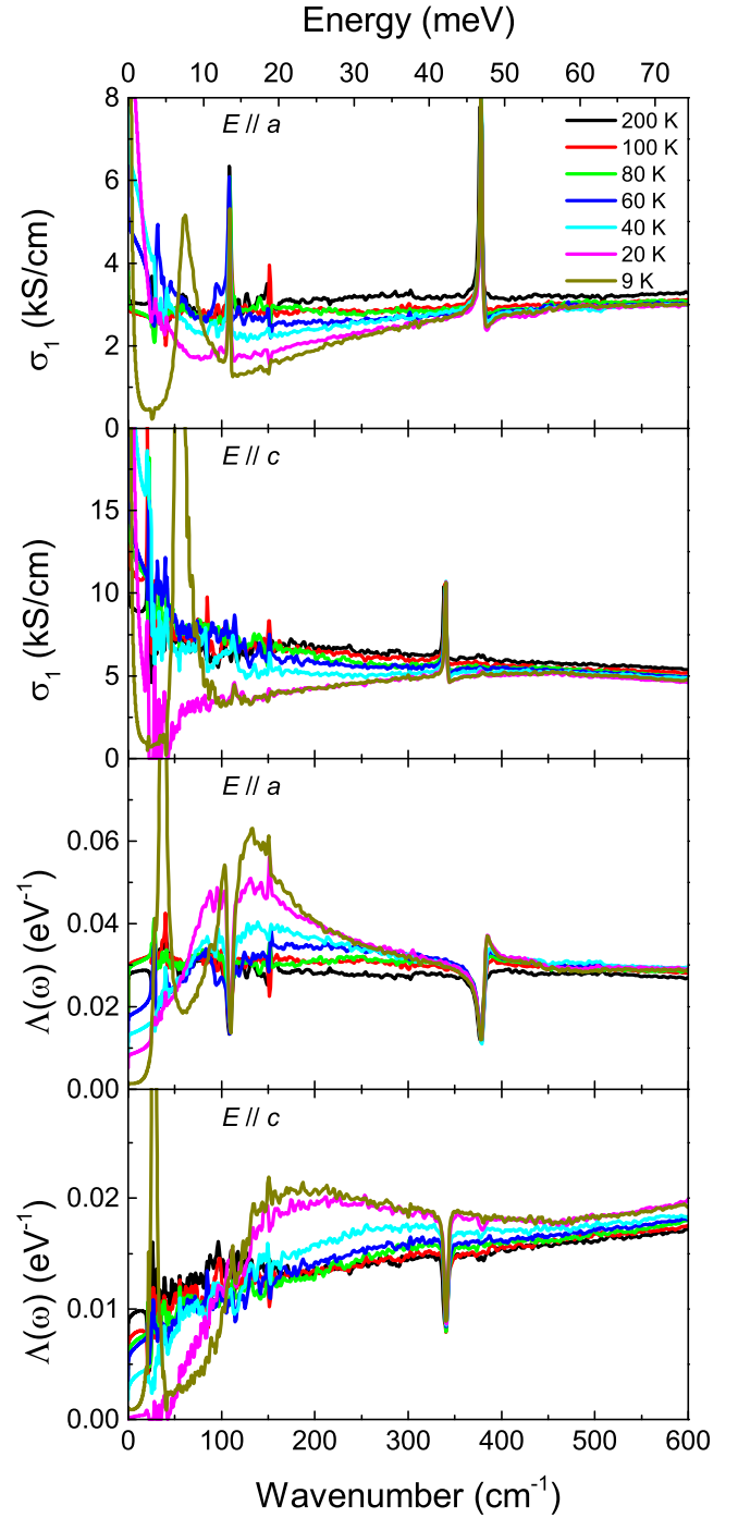
Figure 3. (Color online) Optical conductivity (top) and energy loss function (bottom) of URu 2 Si 2 single crystal in a -axis and c -axis polarizations for selected temperatures.
