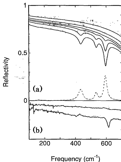
FIG. 1. (a) Theoretical c -axis loss function (dotted, arbitrary units along the vertical axis) and reflectivity (solid). From top to bottom: s -polarized light with a \phi of 45, 30, and 15 degrees relative to the surface normal. Lowest three curves: p polarized, same angles in reverse order. (b) Reflectivity of \text{Tl}_2\text{Ba}_2\text{Ca}_2\text{Cu}_3\text{O}_{10} for s (upper curve) and p -polarized light (lower curve) taken with \phi = 45 degrees.
