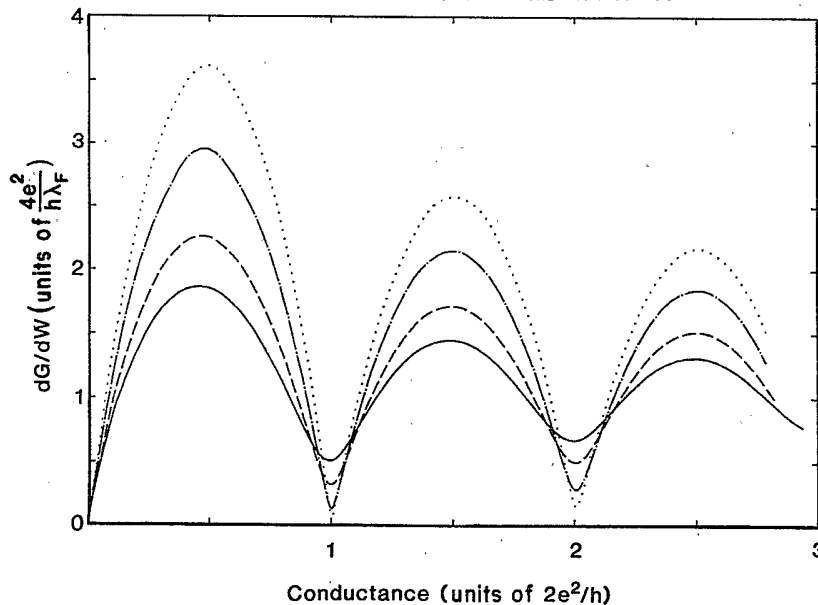
FIG. 3. First derivative of the conductance with respect to kW/\pi vs G for a number of channel lengths. Solid curve: L=0 ; dashed curve: L=0.13\lambda_F ; dash-dotted curve: L=0.25\lambda_F ; dotted curve: L=0.35\lambda_F .
