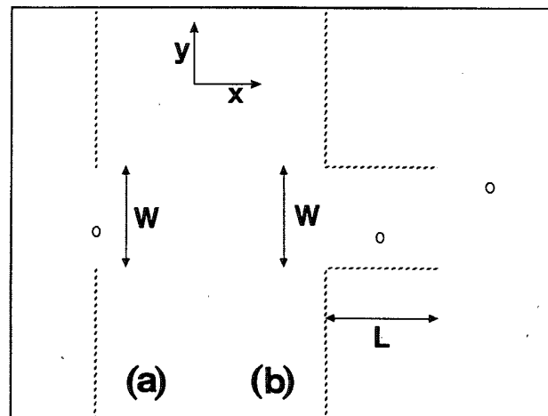
FIG. 1. Geometry for a constriction of (a) zero length and for a constriction of (b) finite length L . Impurities can be incorporated in the constriction on positions such as those indicated by the circles.
