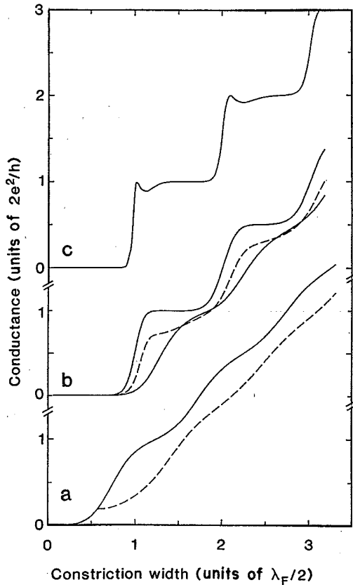
FIG. 2. Conductance vs constriction width. (a) L=0 . Solid and dashed curve: constriction without and with impurity. (b) L=0.48\lambda_F . Upper solid curve: channel without impurity; lower solid curve: impurity inside the constriction ( x=0.32\lambda_F , y=0.32\lambda_F ); dashed curve: impurity outside the constriction ( x=0.57\lambda_F , y=0.32\lambda_F ). (c) L=0.99\lambda_F .
