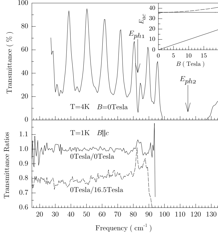
Fig. 3. Upper panel: FIR transmittance at T=4\text{K} , dominated by interference fringes (sample thickness d = 125\mu\text{m} ). The arrows indicate phonon absorption lines. Inset: Magnetic field dependence of the acoustic magnon modes in the spin-flop phase (Solid lines: B \parallel ab , dashed line: B \parallel c ). Lower panel: Ratios of measured transmittance at T=1\text{K} for B \parallel c (Solid line: zero field/zero field, dashed line: zero field/16.5 Tesla).
