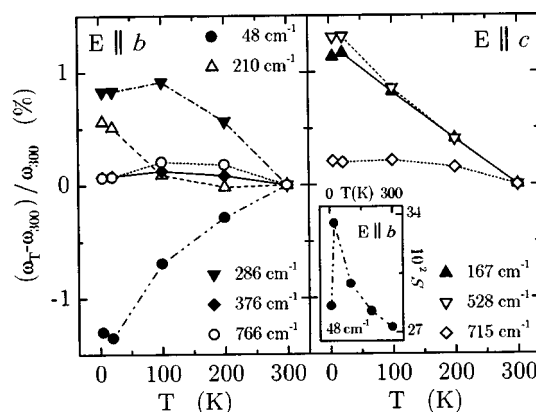
FIG. 4. Temperature dependence of the frequency shift (in percent) of the transverse optical phonons observed for E\parallel b and E\parallel c on the pure single crystal of \text{CuGeO}_3 . In the inset the oscillator strength S of the mode detected at 48\text{ cm}^{-1} , for E\parallel b , is plotted versus the temperature.
