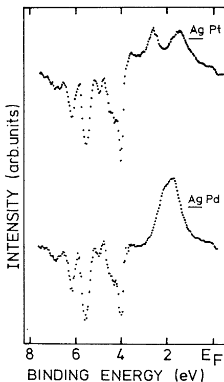
FIG. 8. Difference UPS spectra: AgPd-Ag and AgPt-Ag.
