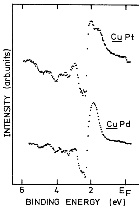
FIG. 7. Difference UPS spectra: CuPd-Cu and CuPt-Cu.
