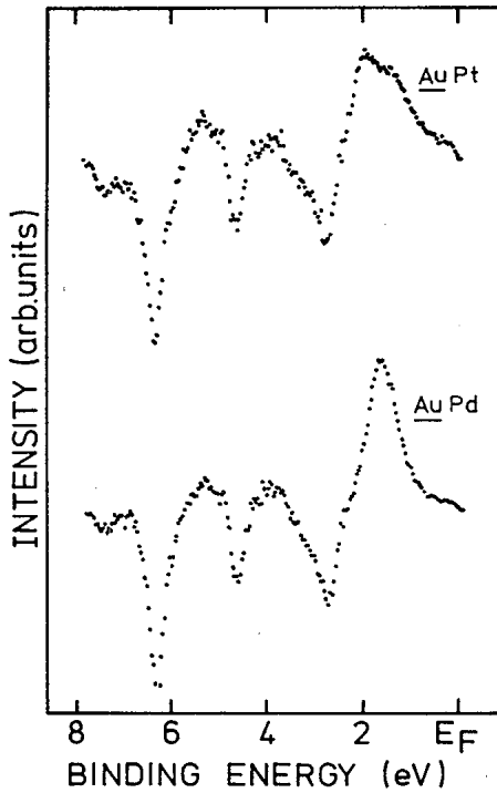
FIG. 9. Difference UPS spectra: AuPd-Au and AuPt-Au .
