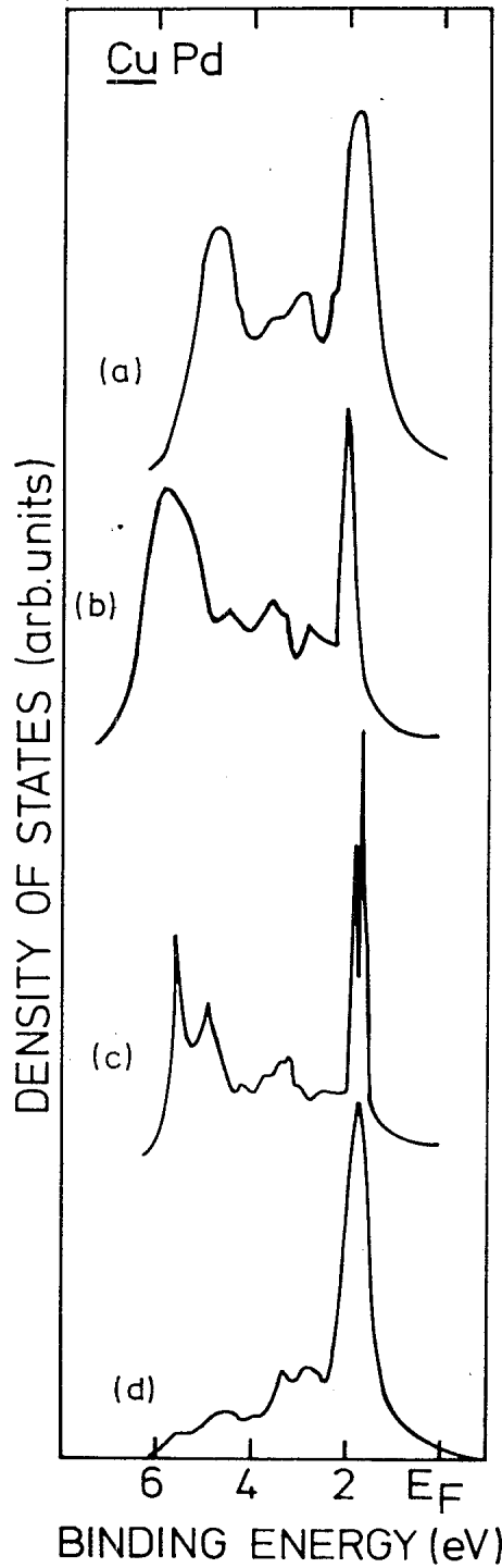
FIG. 17. Local DOS at a Pd site in copper: (a) Ref. 25, (b) Ref. 41, (c) Ref. 5, and (d) this work.
