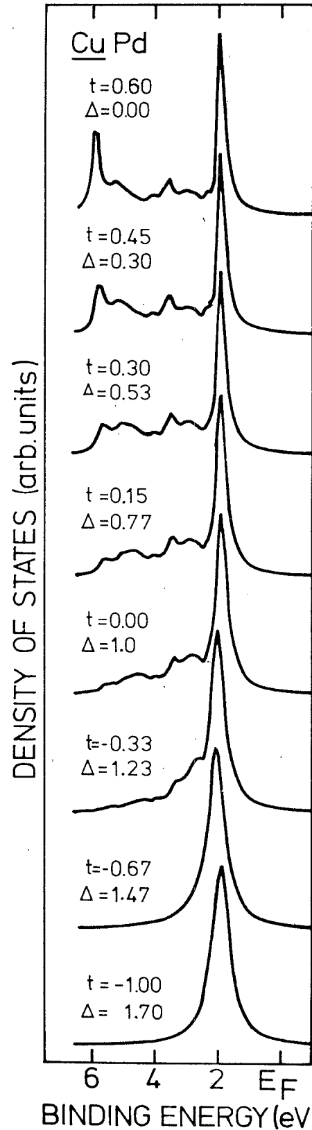
FIG. 18. Local d DOS at a Pd site in CuPd for some parameter values of the Pd- d -Cu- d transfer matrix element.
